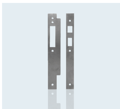
240mm Forend & Strike Plate For EL7200 911.38.416 MYR72
