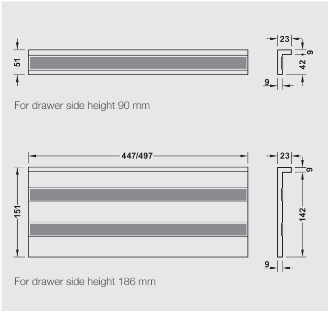
Designer strip, black, open-pored, drawer side height 90mm
