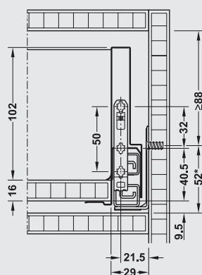
Internal installation height
