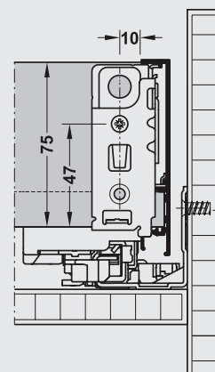
Rear panel drilling dimensions
