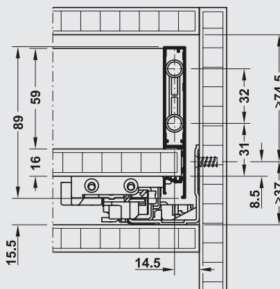
Internal installation height
