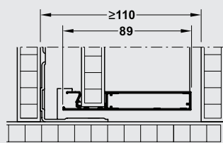
Drawer side height 89 mm
