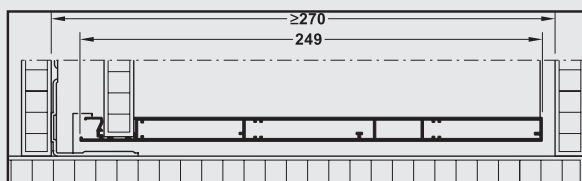
Drawer side height 249 mm
