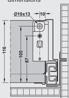
Rear panel installation dimensions
